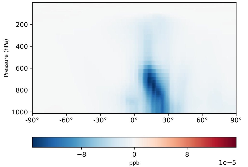
gchp-c24-1Mon-14.7.0-alpha.17_- gchp-c24-1Mon-14.7.0-alpha.16 (Dev) 1x1.25 regrided from c24
