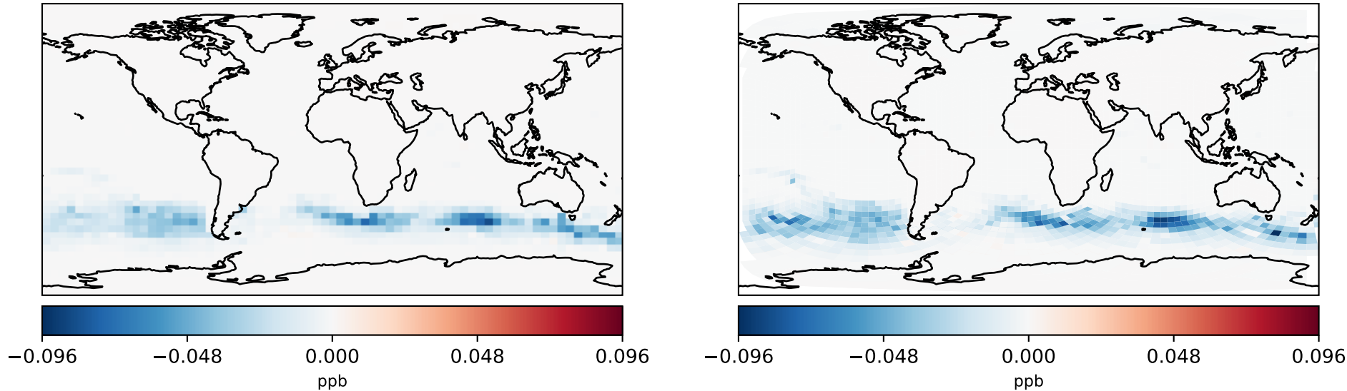
gcc-4x5-1Mon-14.7.0-alpha.17_-_gcc-4x5-1Mon-14.7.0-alpha.16 (Ref) 4.0x5.0 gchp-c24-1Mon-14.7.0-alpha.17_-_gchp-c24-1Mon-14.7.0-alpha.16 (Dev) c24
