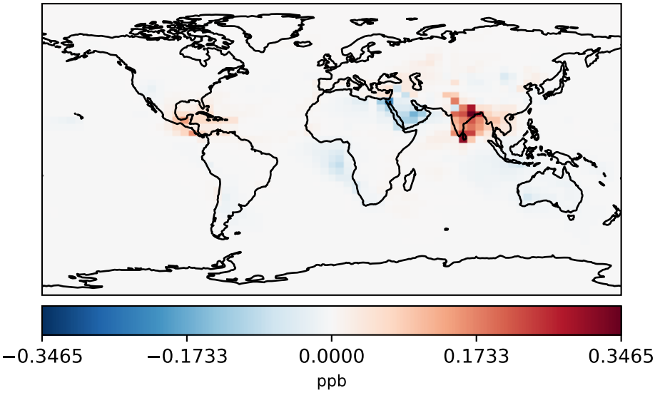
gcc-4x5-1Mon-14.7.0-alpha.17_-_gcc-4x5-1Mon-14.7.0-alpha.16 (Ref) 4.0x5.0 gchp-c24-1Mon-14.7.0-alpha.17_-_gchp-c24-1Mon-14.7.0-alpha.16 (Dev) c24
