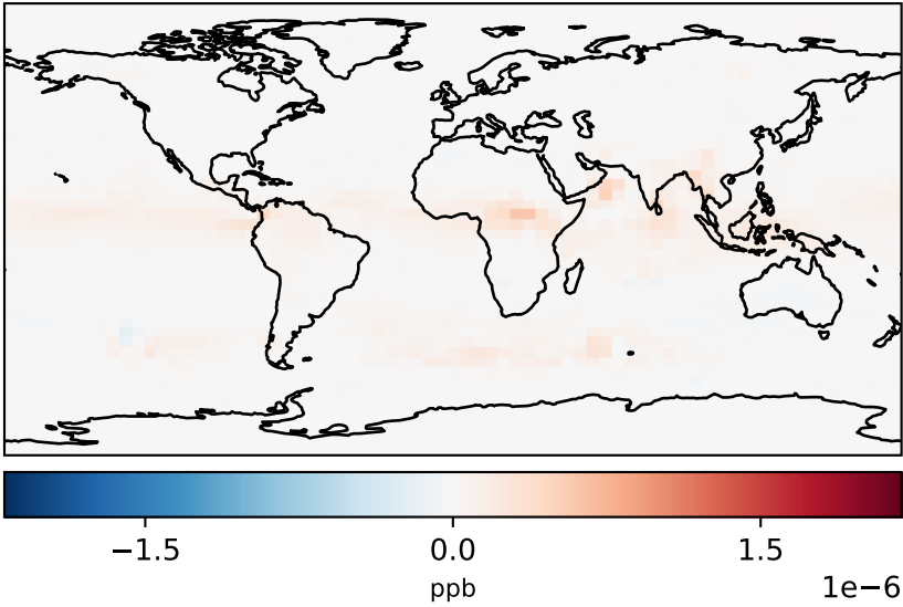
gcc-4x5-1Mon-14.7.0-alpha.17_-_gcc-4x5-1Mon-14.7.0-alpha.16 (Ref) 4.0x5.0 gchp-c24-1Mon-14.7.0-alpha.17_-_gchp-c24-1Mon-14.7.0-alpha.16 (Dev) c24
