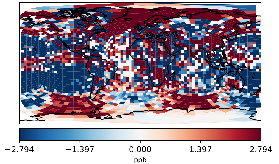
gchp-c24-1Mon-14.7.0-alpha.2_-_gchp-c24-1Mon-14.7.0-alpha.1 (Dev) c24
