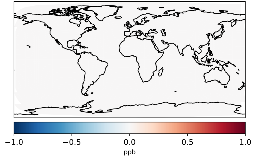
gchp-c24-1Mon-14.7.0-alpha.2_-_gchp-c24-1Mon-14.7.0-alpha.1 (Dev) c24
