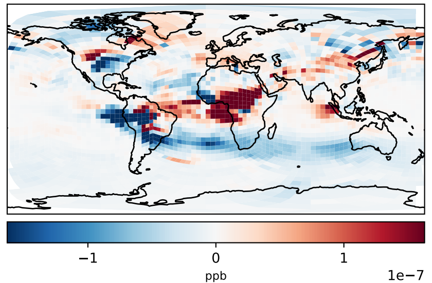
gchp-c24-1Mon-14.7.0-alpha.2_-_gchp-c24-1Mon-14.7.0-alpha.1 (Dev) c24
