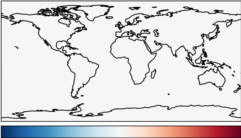
gcc-4x5-1Mon-14.7.0-alpha.17 - gcc-4x5-1Mon-14.6.3 (Ref) 4.0x5.0
