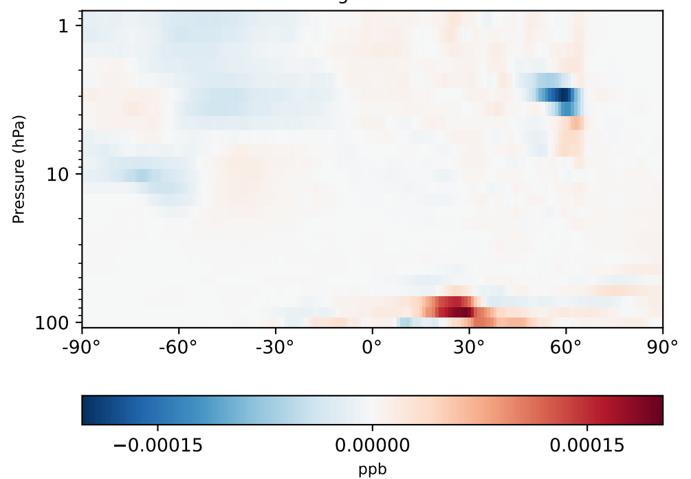
gchp-c24-1Mon-14.6.3 - gchp-c24-1Mon-14.6.2 (Dev) 1x1.25 regriidd from c24
