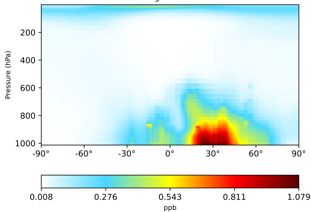
gchp-c24-1Mon-14.7.0-alpha.9 (Ref) 1x1.25 regrided from c24
