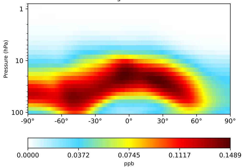
gchp-c24-1Mon-14.7.0-alpha.9 (Ref) 1x1.25 regrided from c24
