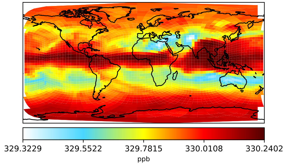
gchp-c24-1Mon-14.7.0-alpha.9 (Ref) c24
