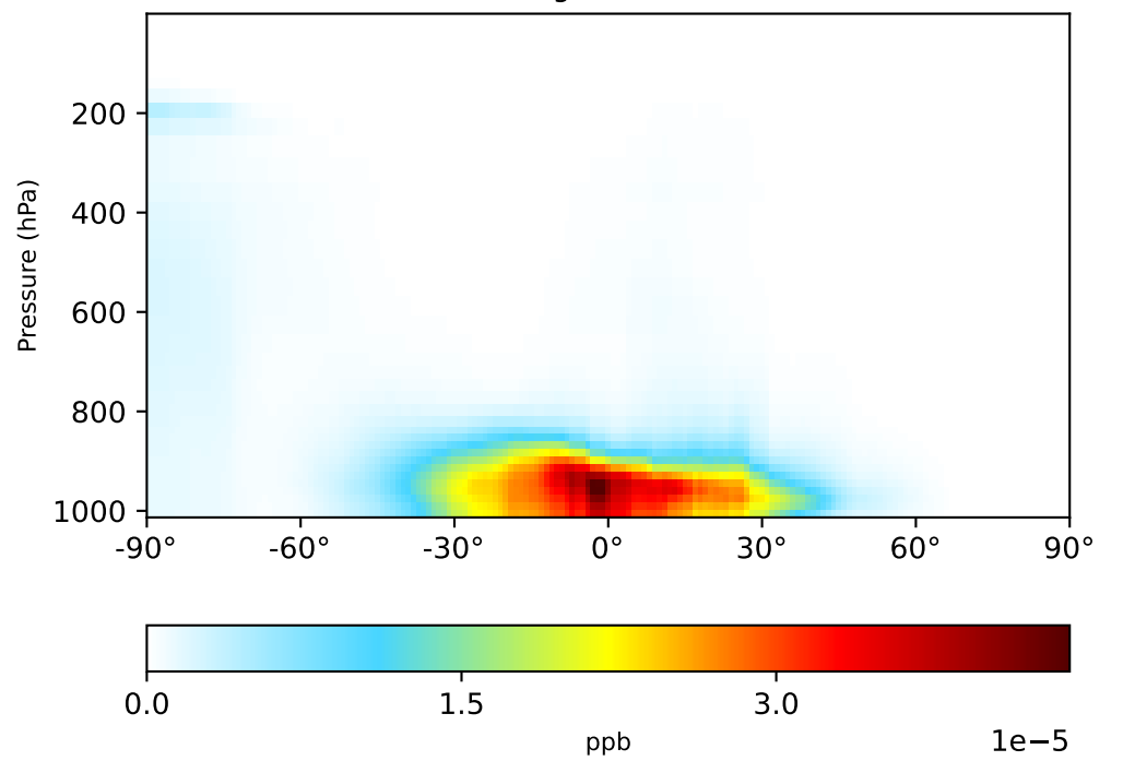
gchp-c24-1Mon-14.7.0-alpha.10 (Dev) 1x1.25 regridded from c24
