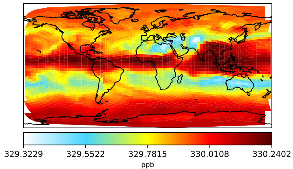
gchp-c24-1Mon-14.7.0-alpha.8 (Ref) c24
