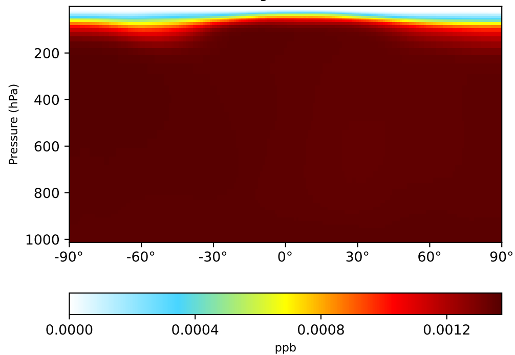
gchp-c24-1Mon-14.7.0-alpha.8 (Ref) 1x1.25 regrided from c24
