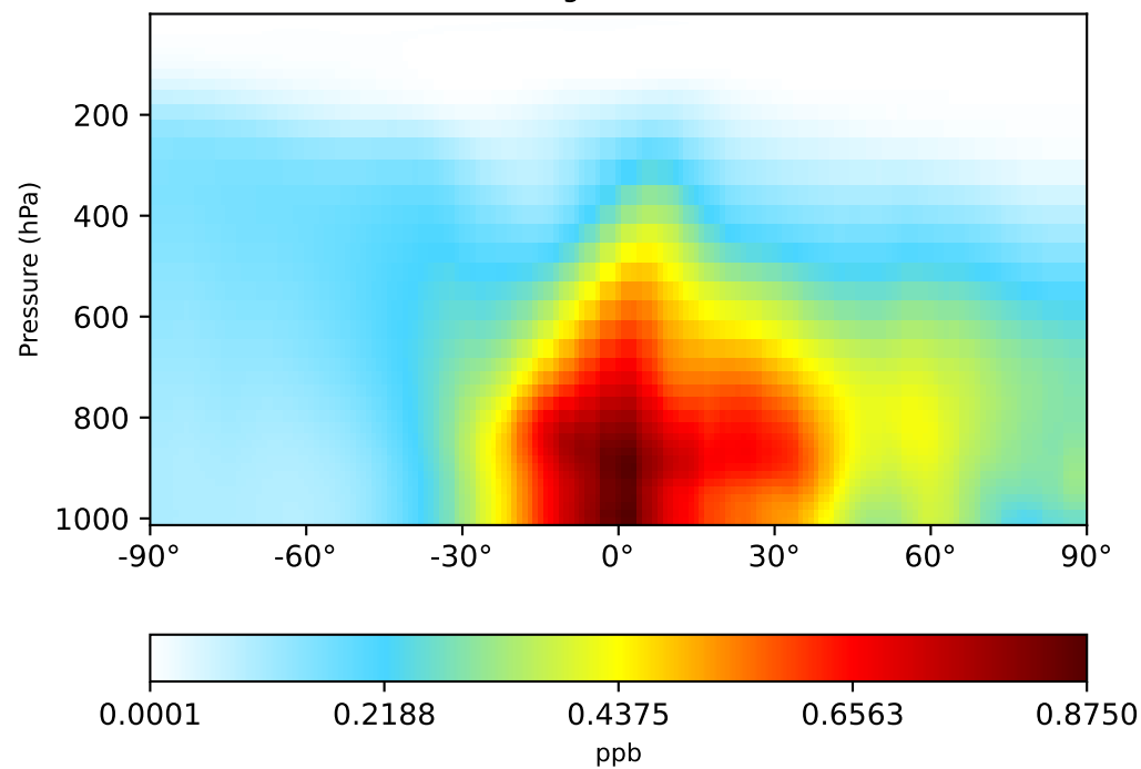
gchp-c24-1Mon-14.7.0-alpha.7 (Ref) 1x1.25 regridded from c24
