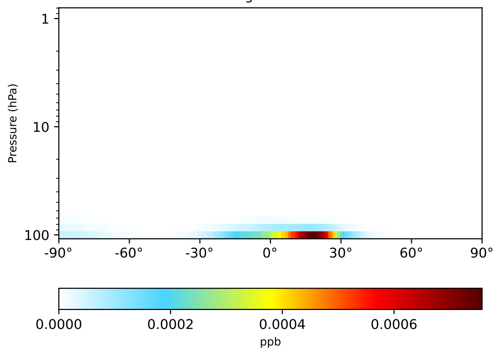
gchp-c24-1Mon-14.7.0-alpha.8 (Dev) 1x1.25 regridded from c24
