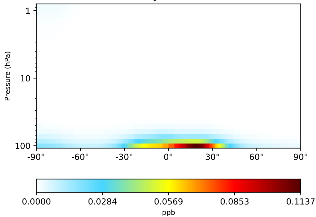
gchp-c24-1Mon-14.7.0-alpha.7 (Ref) 1x1.25 regridded from c24
