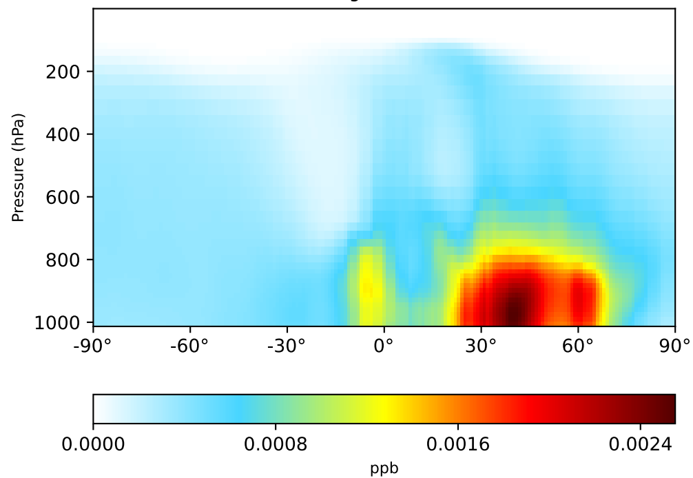
gchp-c24-1Mon-14.7.0-alpha.6 (Ref) 1x1.25 regrided from c24
