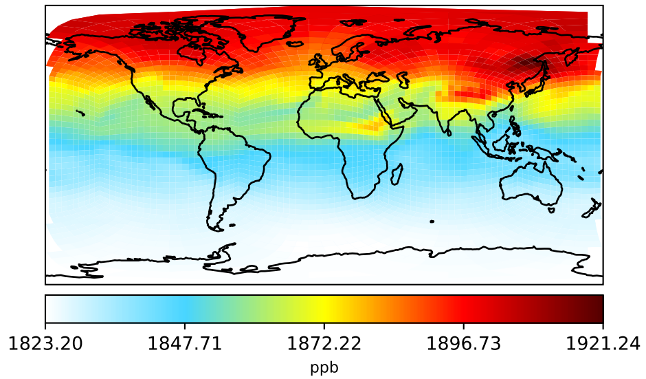
gchp-c24-1Mon-14.7.0-alpha.5 (Ref) c24
