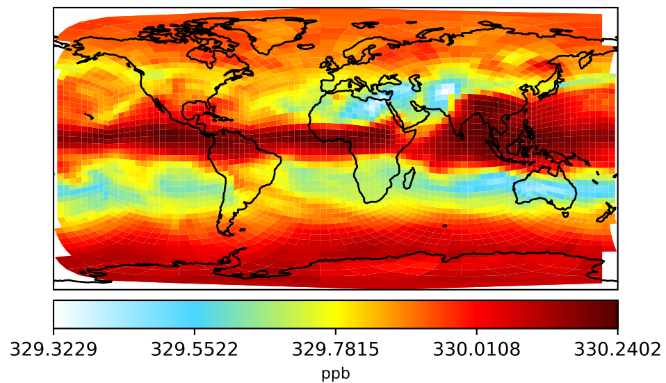
gchp-c24-1Mon-14.7.0-alpha.5 (Ref) c24
