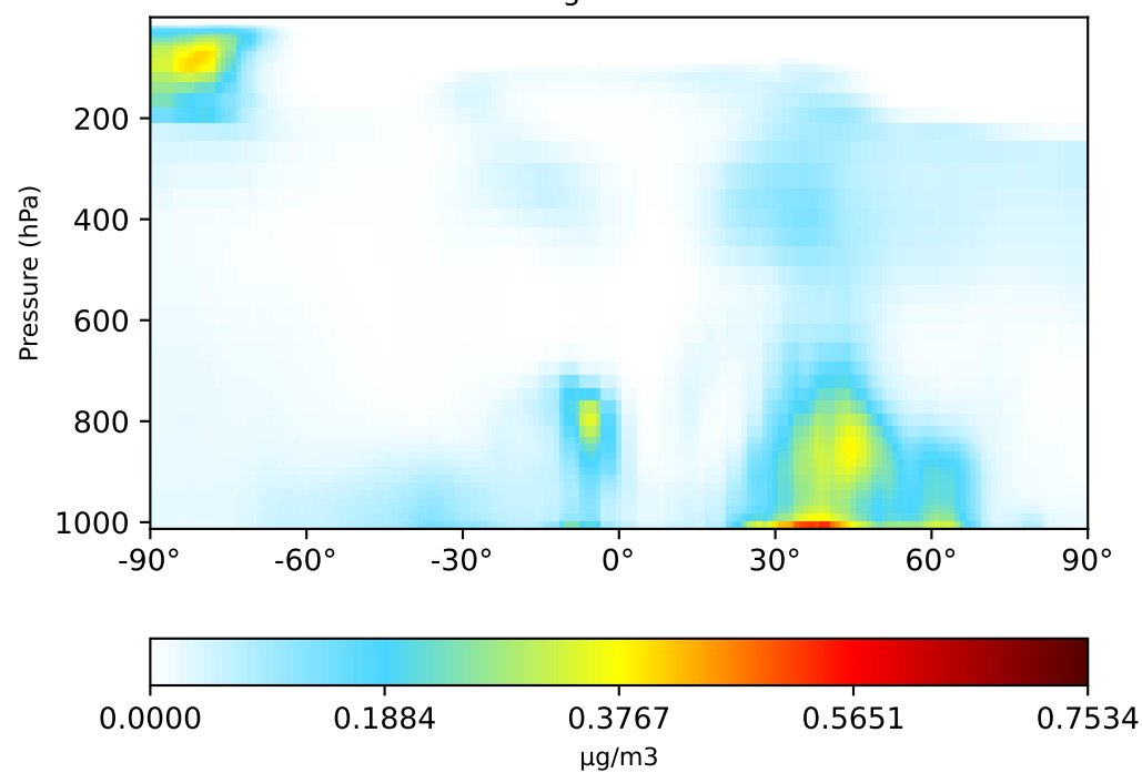
gchp-c24-1Mon-14.7.0-alpha.5 (Ref) 1x1.25 regrided from c24
