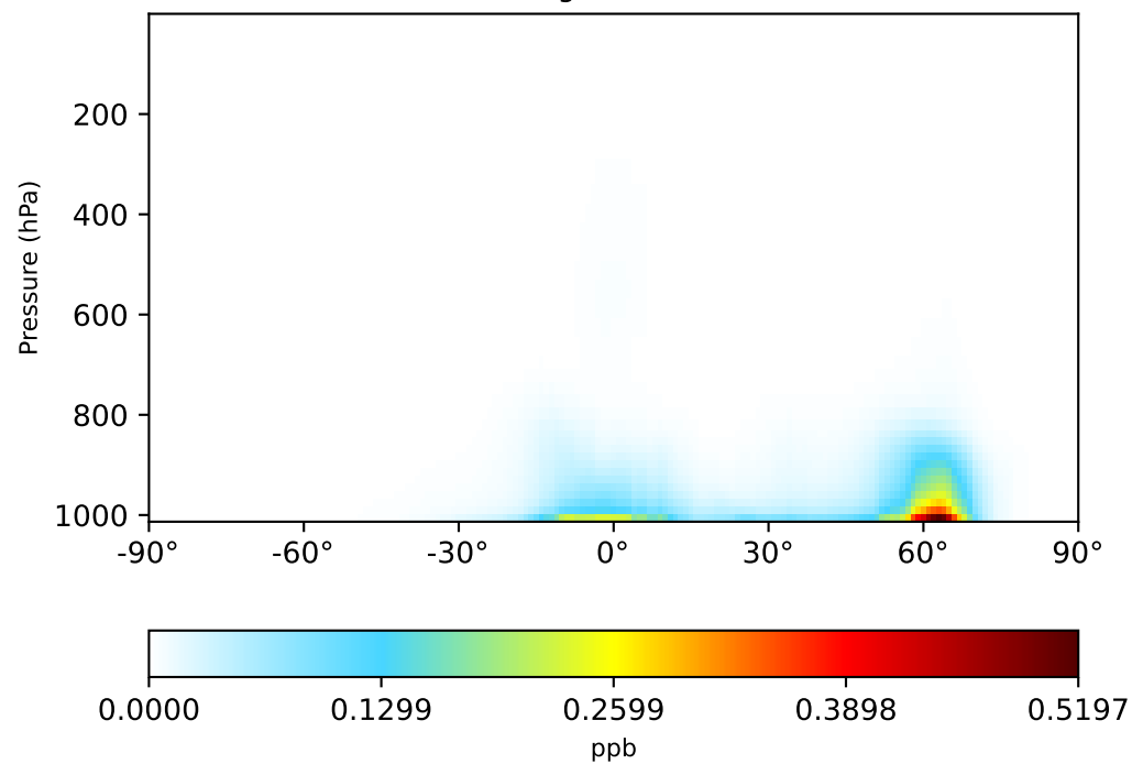
gchp-c24-1Mon-14.7.0-alpha.4 (Ref) 1x1.25 regridded from c24
