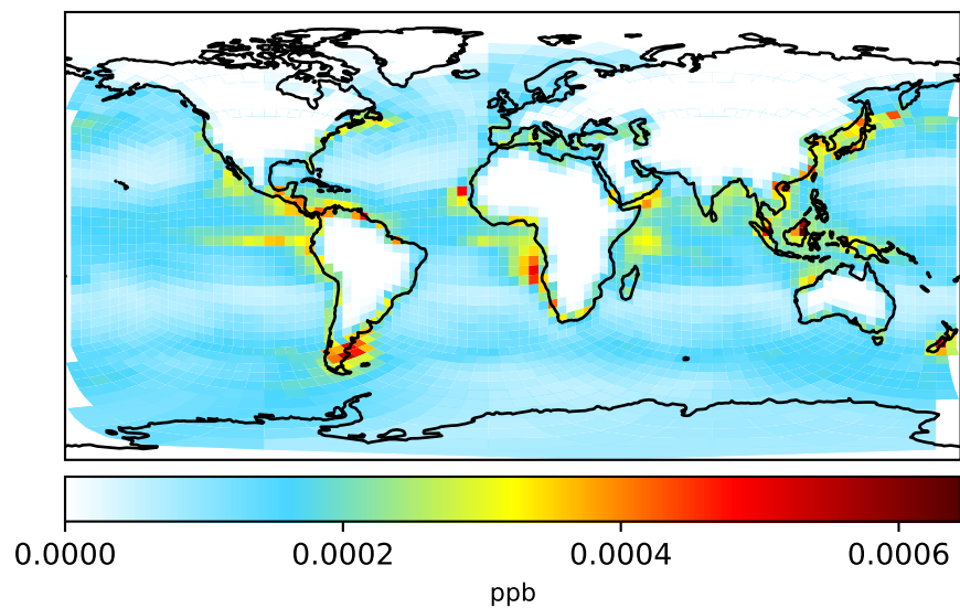
gchp-c24-1Mon-14.7.0-alpha.4 (Ref) c24
