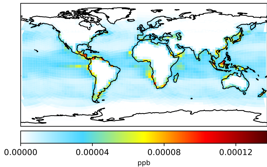
gchp-c24-1Mon-14.7.0-alpha.4 (Ref) c24
