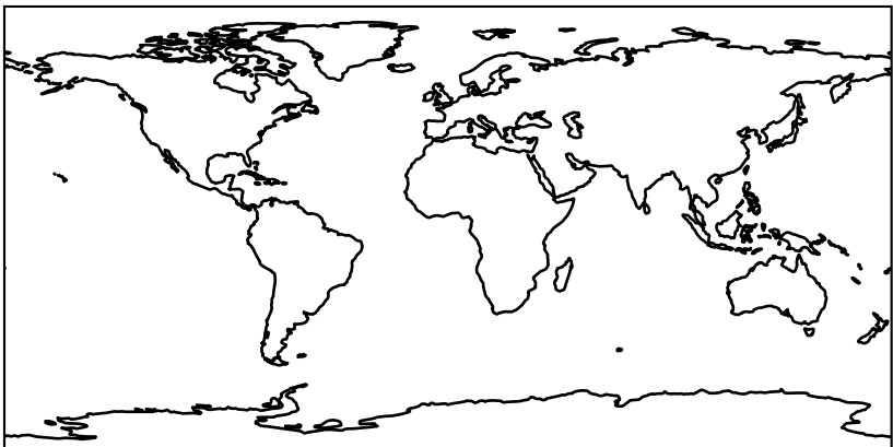
gchp-c24-1Mon-14.7.0-alpha.4 (Ref) c24
