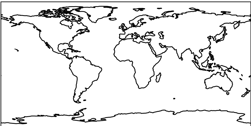
gchp-c24-1Mon-14.7.0-alpha.5 (Dev) c24
