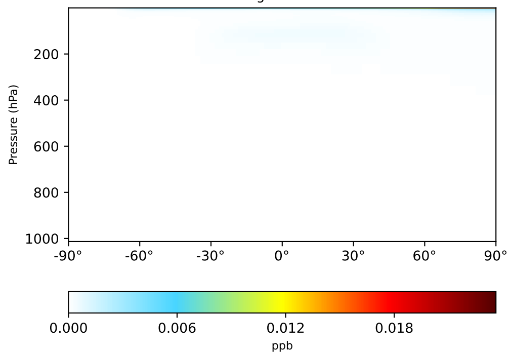
gchp-c24-1Mon-14.7.0-alpha.4 (Ref) 1x1.25 regrided from c24
