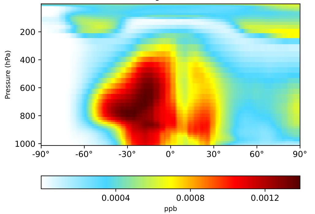
gchp-c24-1Mon-14.7.0-alpha.5 (Dev) 1x1.25 regrided from c24
