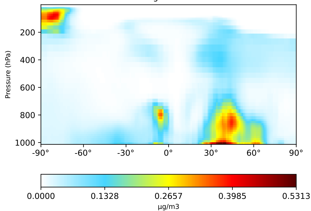
gchp-c24-1Mon-14.7.0-alpha.4 (Ref) 1x1.25 regrided from c24
