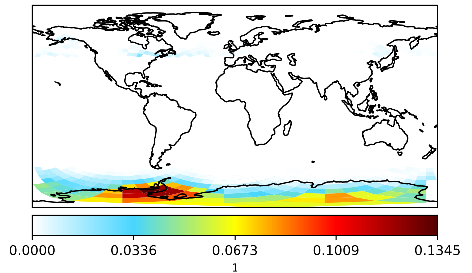
gchp-c24-1Mon-14.7.0-alpha.5 (Dev) c24
