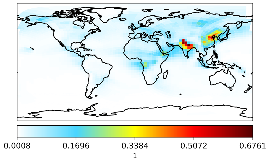
gchp-c24-1Mon-14.7.0-alpha.4 (Ref) c24
