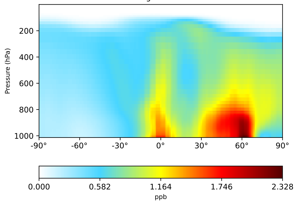
gchp-c24-1Mon-14.7.0-alpha.3 (Ref) 1x1.25 regridded from c24
