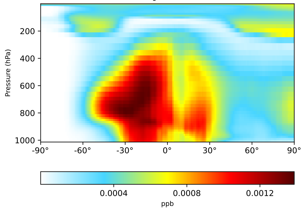
gchp-c24-1Mon-14.7.0-alpha.3 (Ref) 1x1.25 regridded from c24
