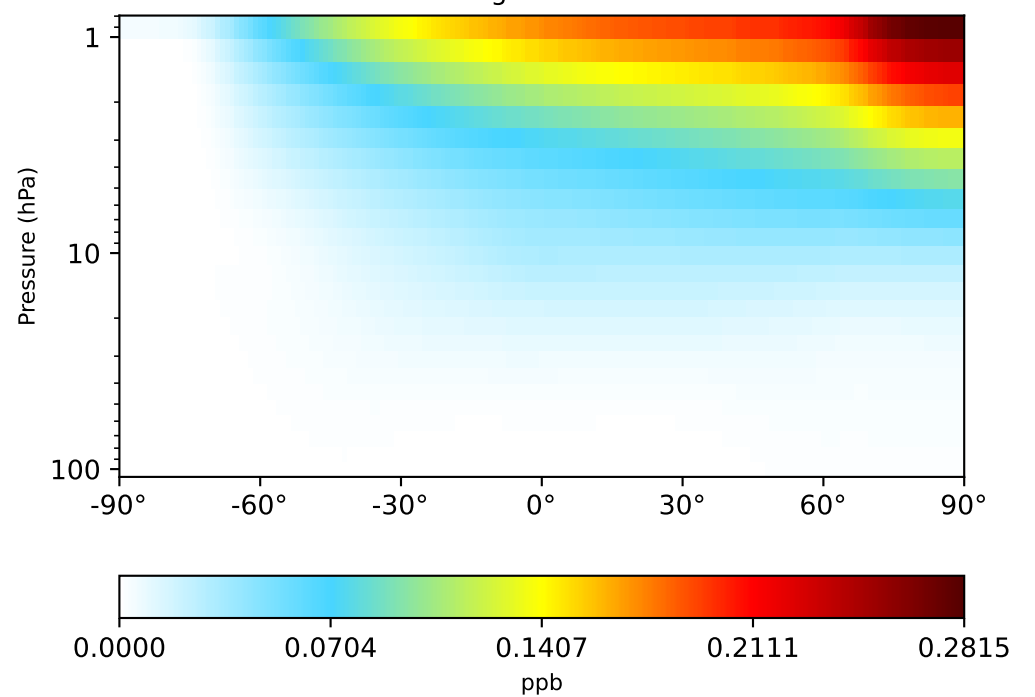
gchp-c24-1Mon-14.7.0-alpha.3 (Dev) 1x1.25 regrided from c24
