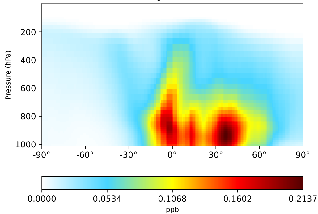
gchp-c24-1Mon-14.7.0-alpha.2 (Ref) 1x1.25 regridded from c24
