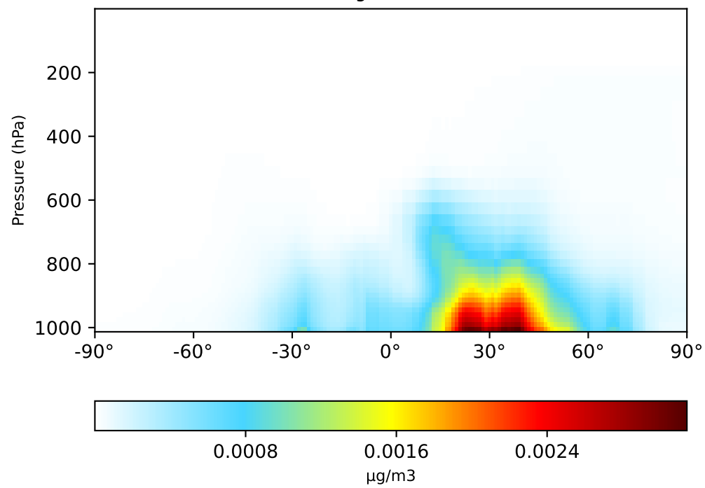
gchp-c24-1Mon-14.7.0-alpha.2 (Ref) 1x1.25 regrided from c24
