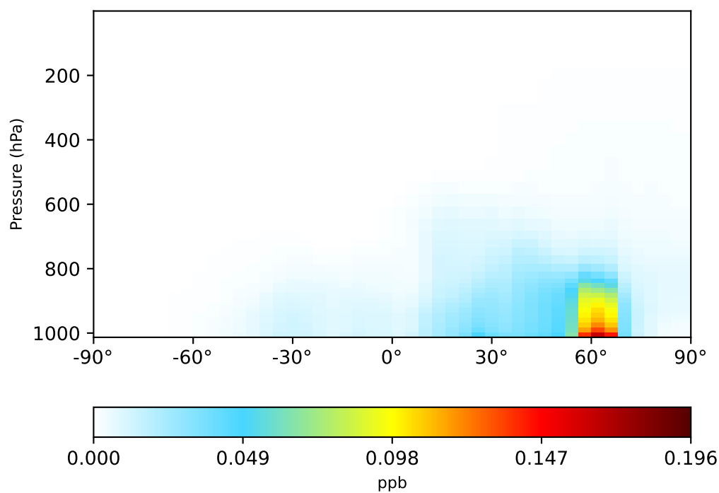
gcc-4x5-1Mon-14.7.0-alpha.2 (Ref) 4.0x5.0
