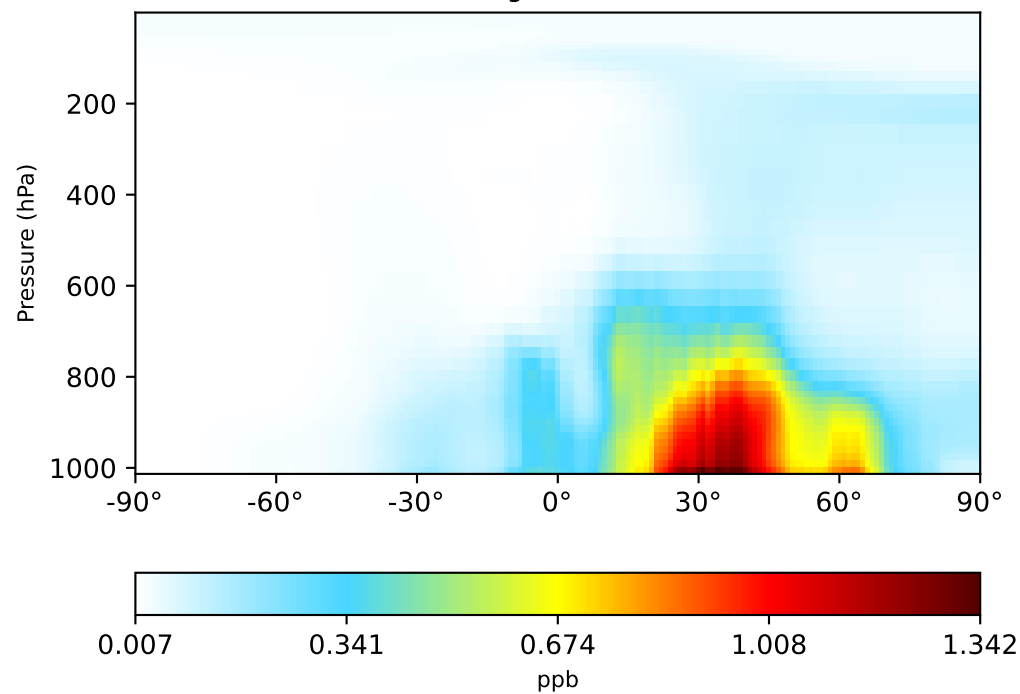
gchp-c24-1Mon-14.7.0-alpha.17 (Ref) 1x1.25 regrided from c24
