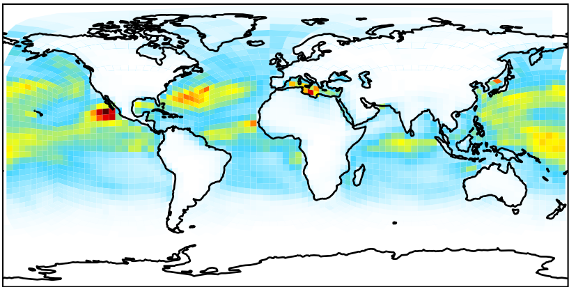
gchp-c24-1Mon-14.7.0-alpha.17 (Ref) c24
