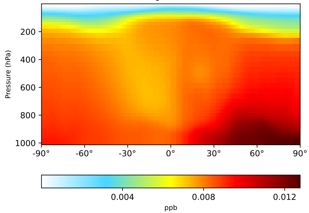
gchp-c24-1Mon-14.7.0-alpha.16 (Ref) 1x1.25 regrided from c24
