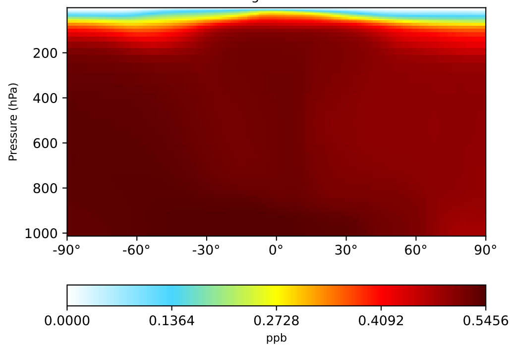
gchp-c24-1Mon-14.7.0-alpha.16 (Ref) 1x1.25 regridded from c24
