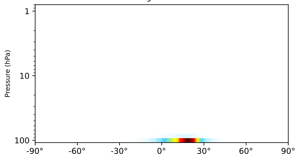
gchp-c24-1Mon-14.7.0-alpha.17 (Dev) 1x1.25 regridded from c24
