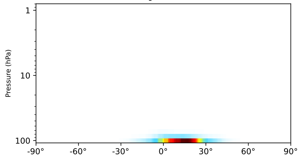
gchp-c24-1Mon-14.7.0-alpha.17 (Dev) 1x1.25 regridded from c24
