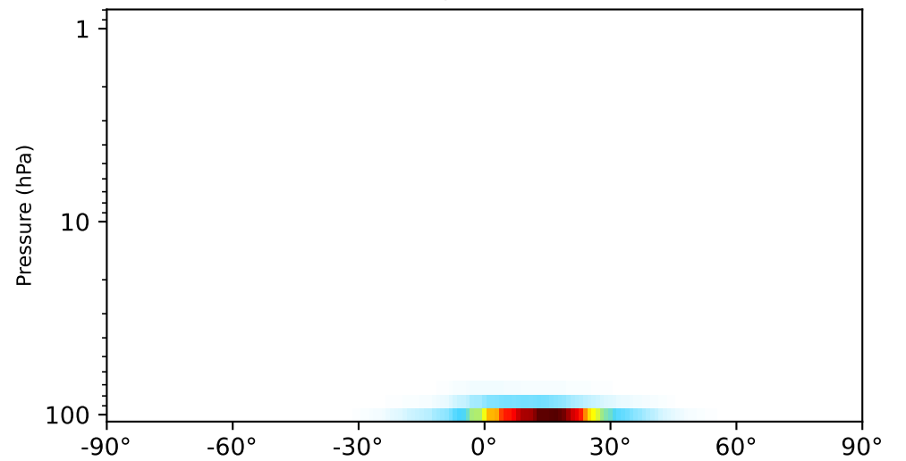
gchp-c24-1Mon-14.7.0-alpha.17 (Dev) 1x1.25 regridded from c24
