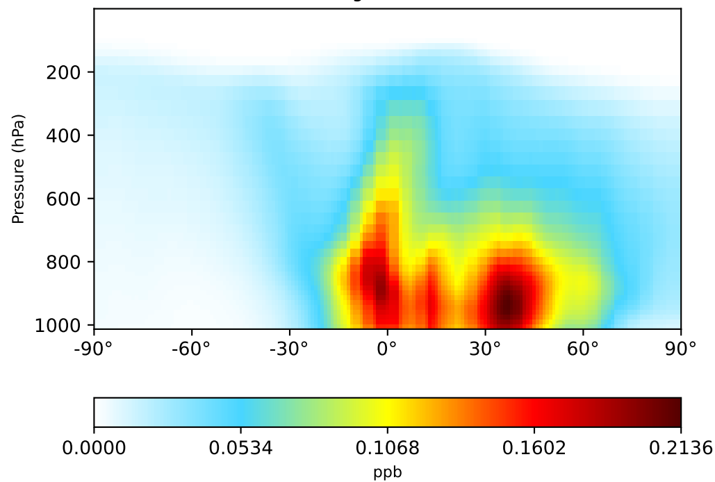
gchp-c24-1Mon-14.7.0-alpha.15 (Ref) 1x1.25 regridded from c24
