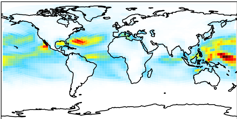
gchp-c24-1Mon-14.7.0-alpha.15 (Ref) c24
