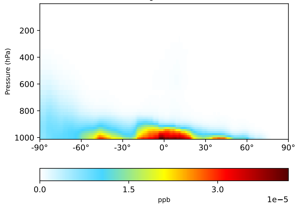
gchp-c24-1Mon-14.7.0-alpha.15 (Ref) 1x1.25 regridded from c24
