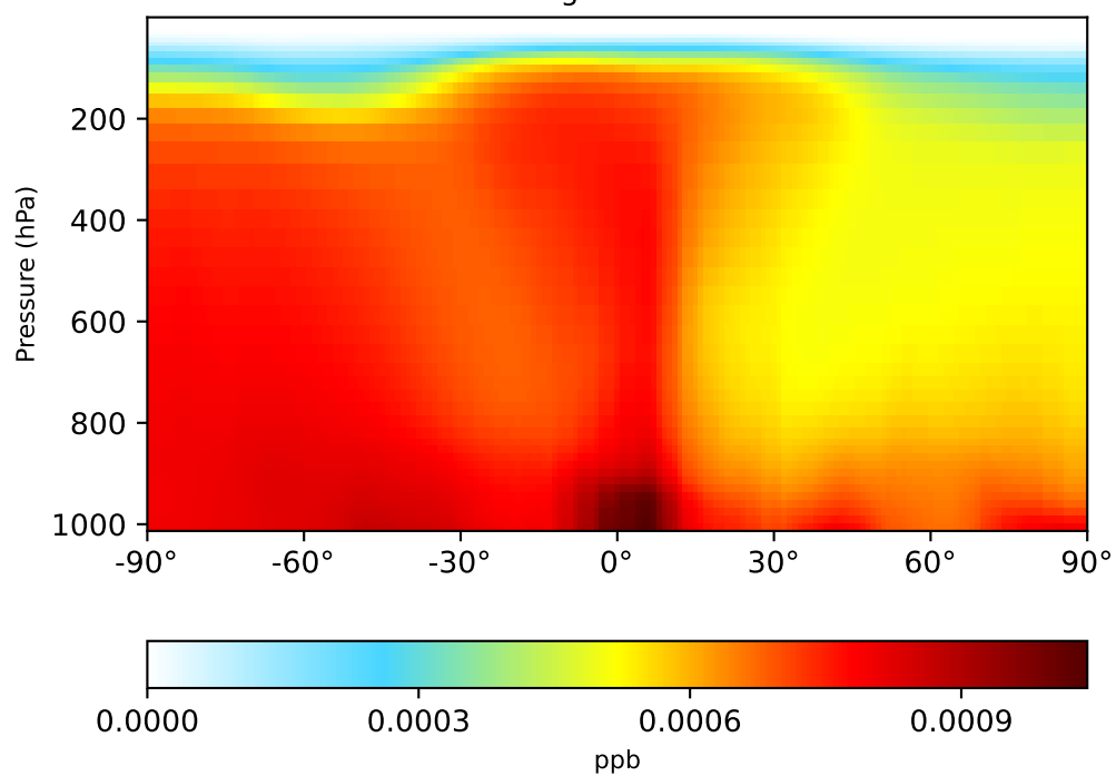
gchp-c24-1Mon-14.7.0-alpha.15 (Dev) 1x1.25 regrided from c24
