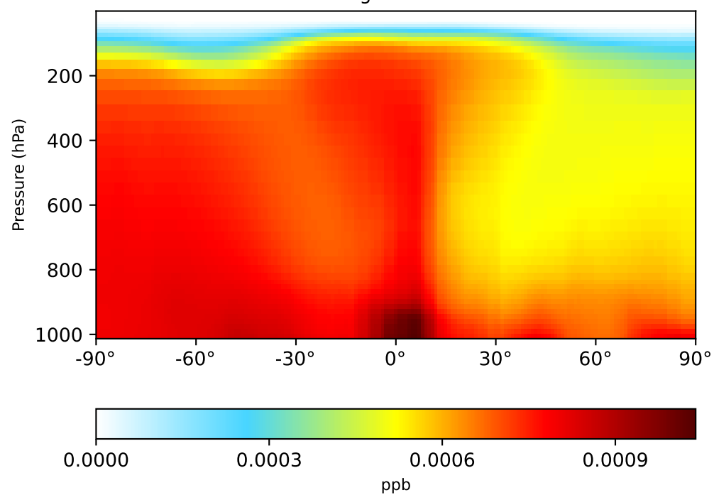
gchp-c24-1Mon-14.7.0-alpha.14 (Ref) 1x1.25 regrided from c24
