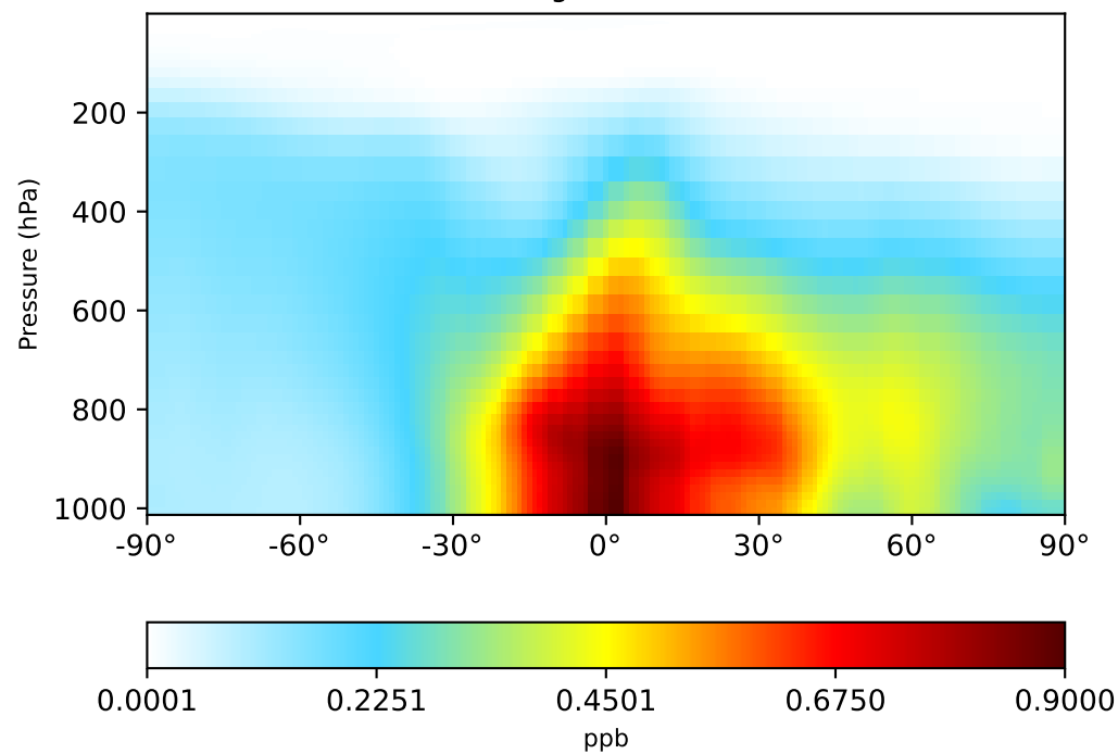
gchp-c24-1Mon-14.7.0-alpha.13 (Ref) 1x1.25 regrided from c24
