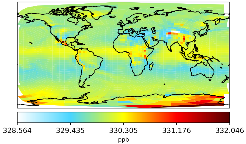
gchp-c24-1Mon-14.7.0-alpha.13 (Ref) c24
