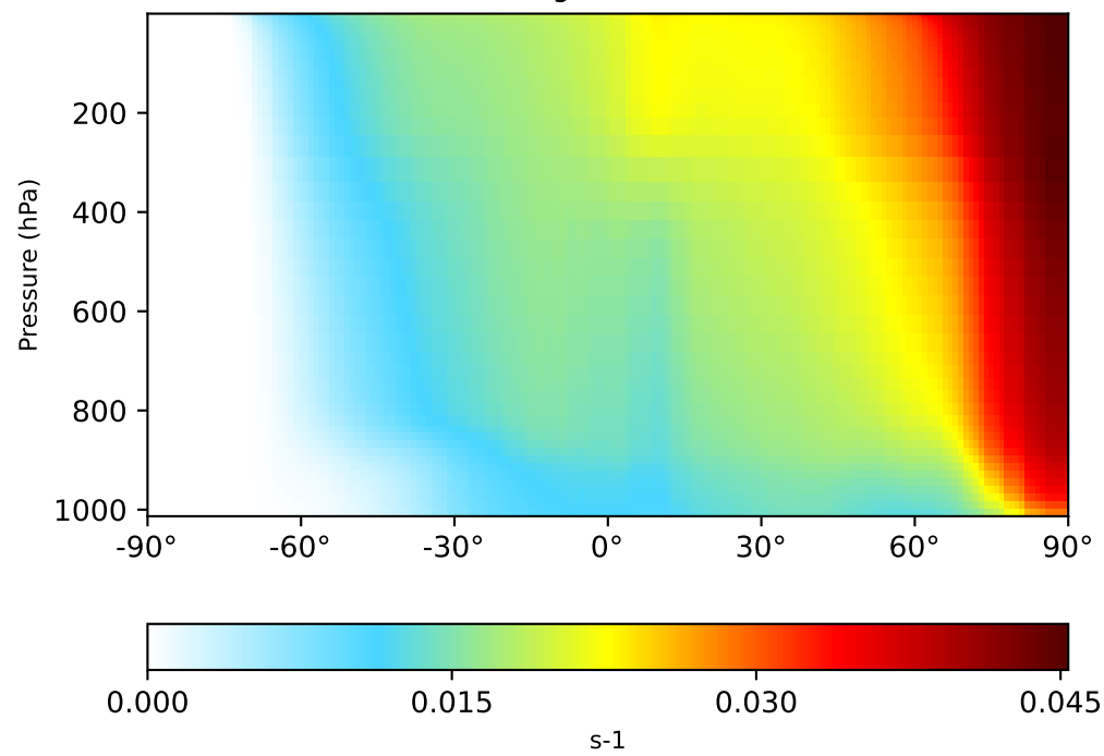
gchp-c24-1Mon-14.7.0-alpha.13 (Ref) 1x1.25 regrided from c24
