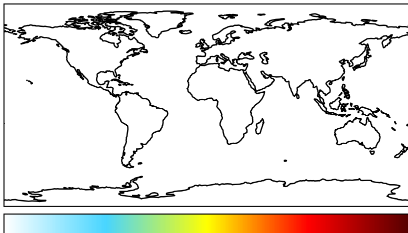
gchp-c24-1Mon-14.7.0-alpha.13 (Ref) c24
