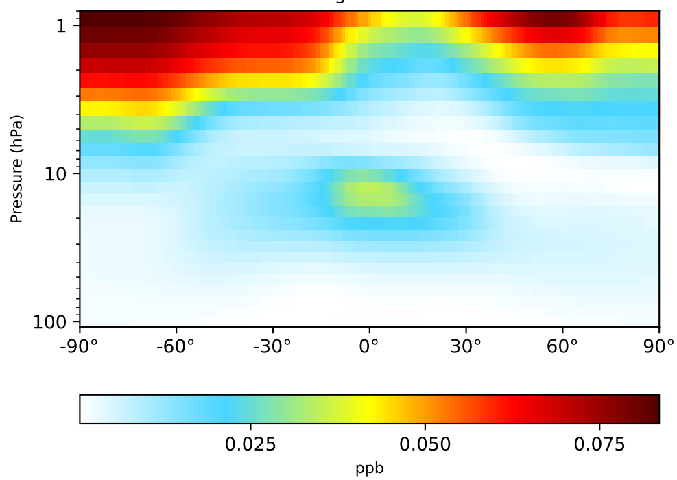
gchp-c24-1Mon-14.7.0-alpha.11 (Ref) 1x1.25 regridded from c24
