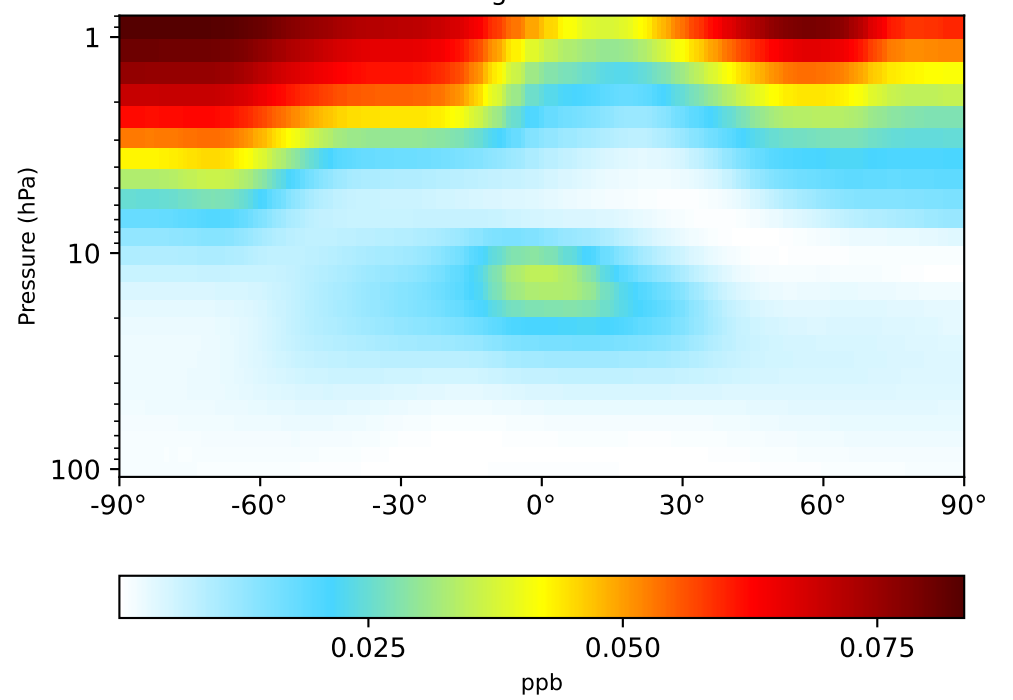
gchp-c24-1Mon-14.7.0-alpha.12 (Dev) 1x1.25 regridded from c24
