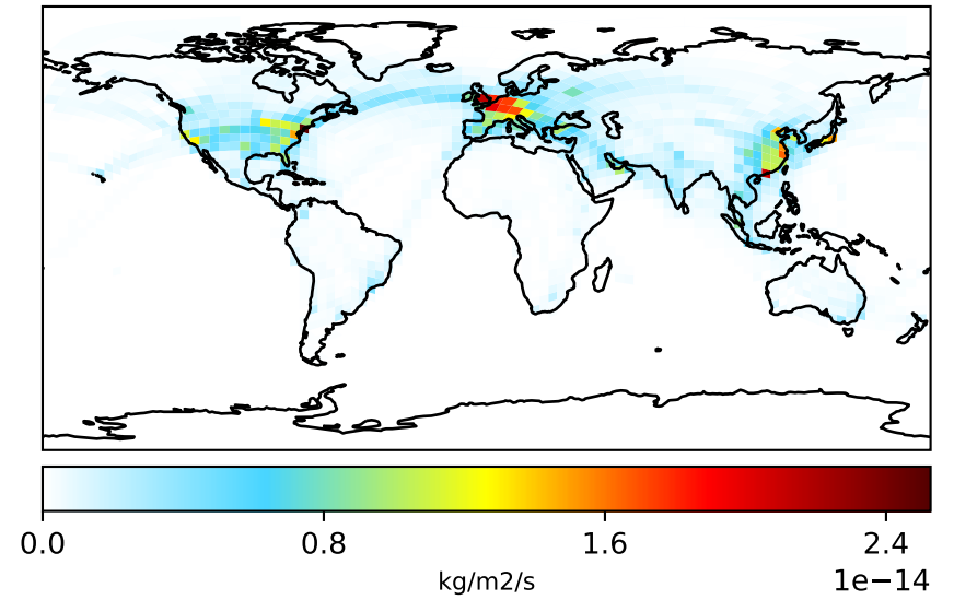
gchp-c24-1Mon-14.7.0-alpha.12 (Dev) c24
