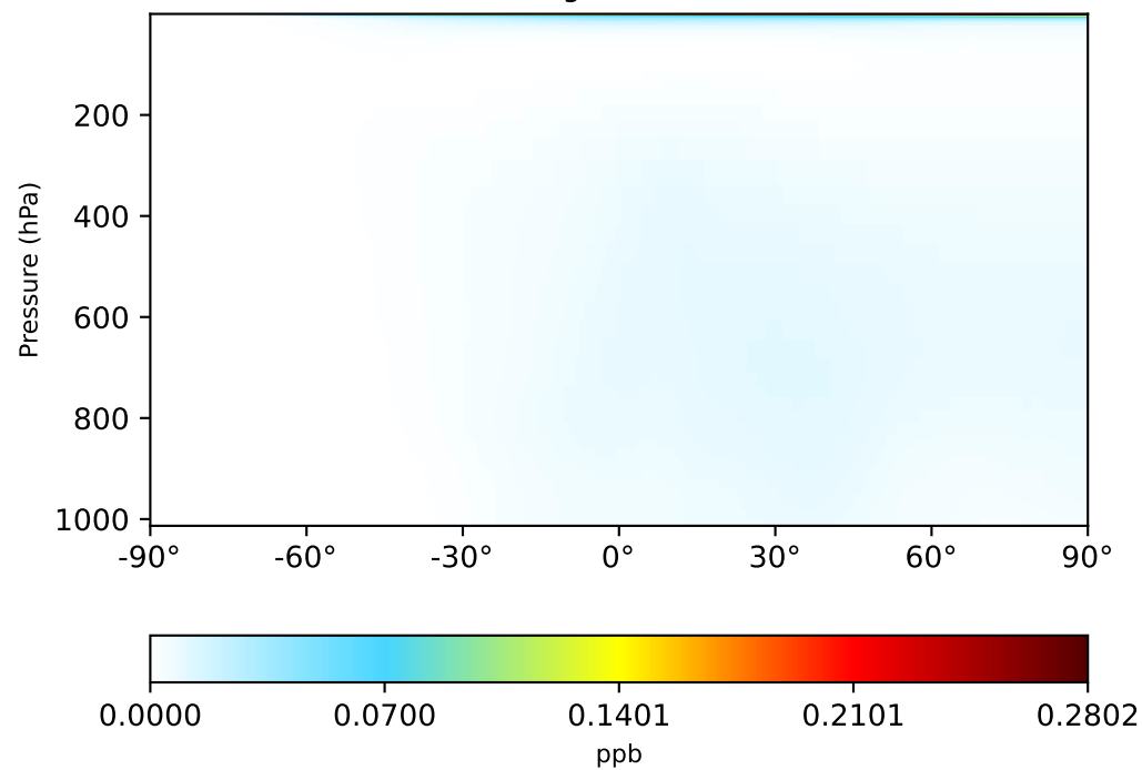
gchp-c24-1Mon-14.7.0-alpha.11 (Ref) 1x1.25 regridded from c24
