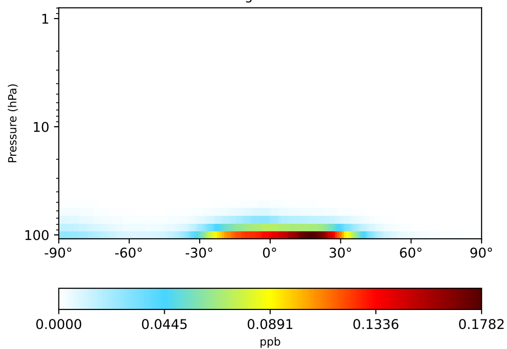
gchp-c24-1Mon-14.7.0-alpha.12 (Dev) 1x1.25 regrided from c24
