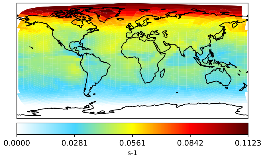
gchp-c24-1Mon-14.7.0-alpha.11 (Ref) c24
