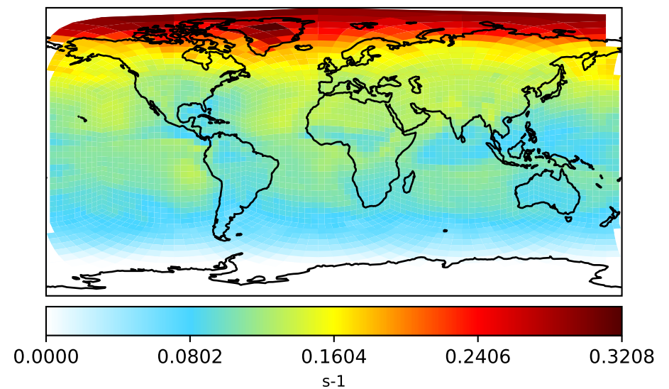
gchp-c24-1Mon-14.7.0-alpha.12 (Dev) c24
