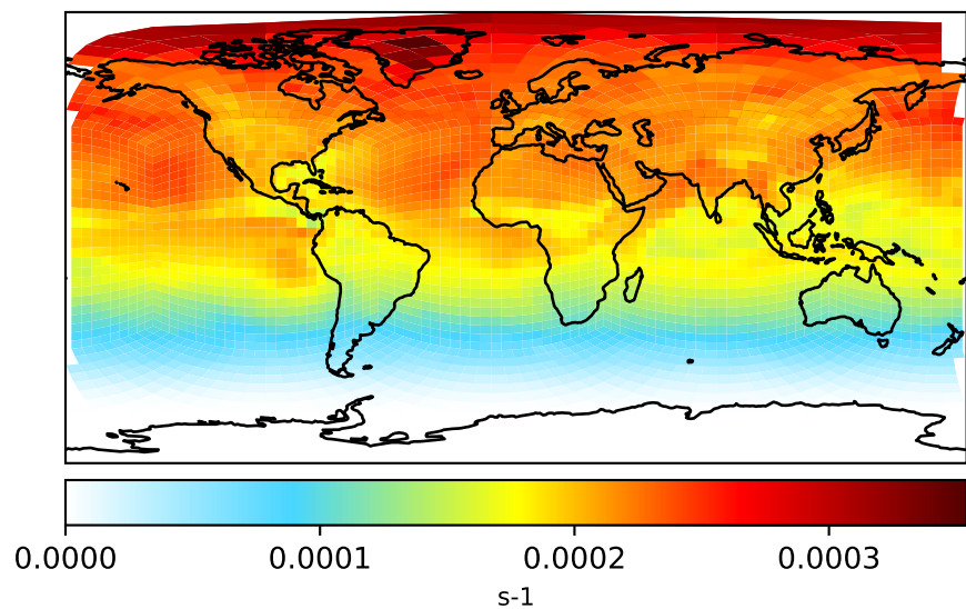
gchp-c24-1Mon-14.7.0-alpha.11 (Ref) c24
