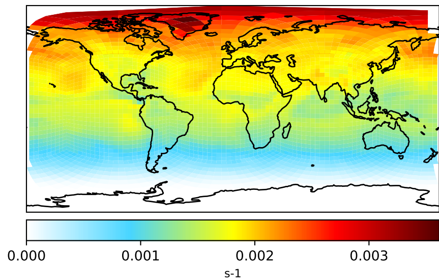
gchp-c24-1Mon-14.7.0-alpha.11 (Ref) c24
