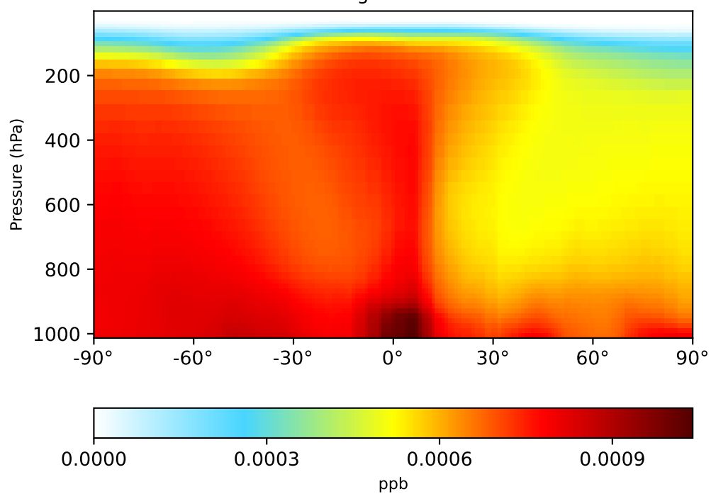
gchp-c24-1Mon-14.7.0-alpha.12 (Dev) 1x1.25 regrided from c24
