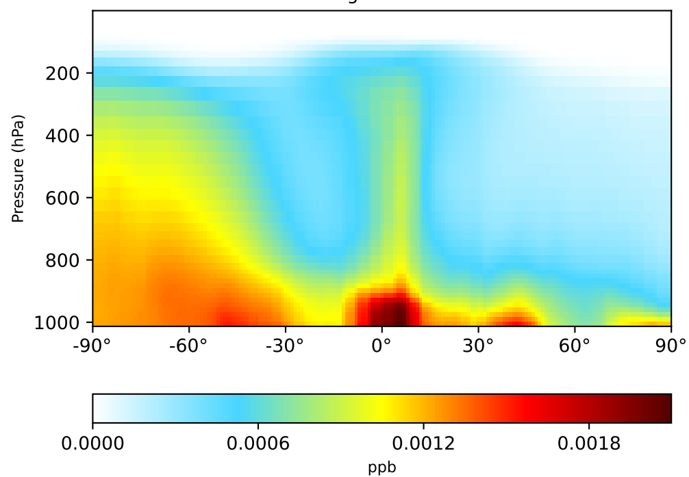
gchp-c24-1Mon-14.7.0-alpha.11 (Ref) 1x1.25 regrided from c24
