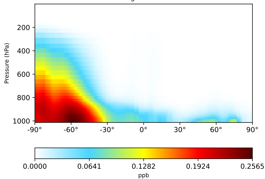
gchp-c24-1Mon-14.7.0-alpha.10 (Ref) 1x1.25 regrided from c24
